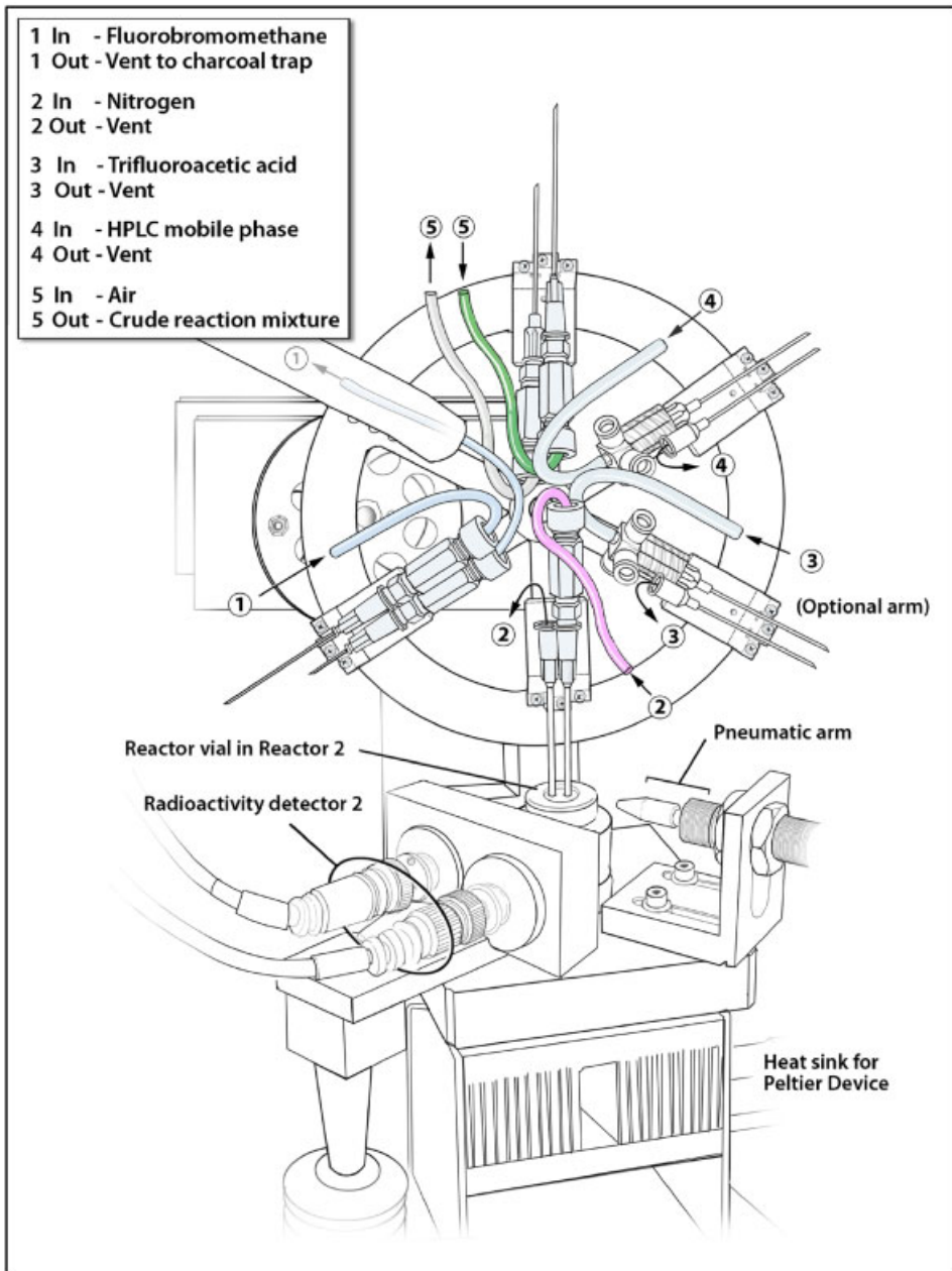
Figure 2. Automated apparatus for entrapment of [ ^{18}\text{F} ]fluorobromomethane for the preparation of [ ^{18}\text{F} ]SPA-RQ
