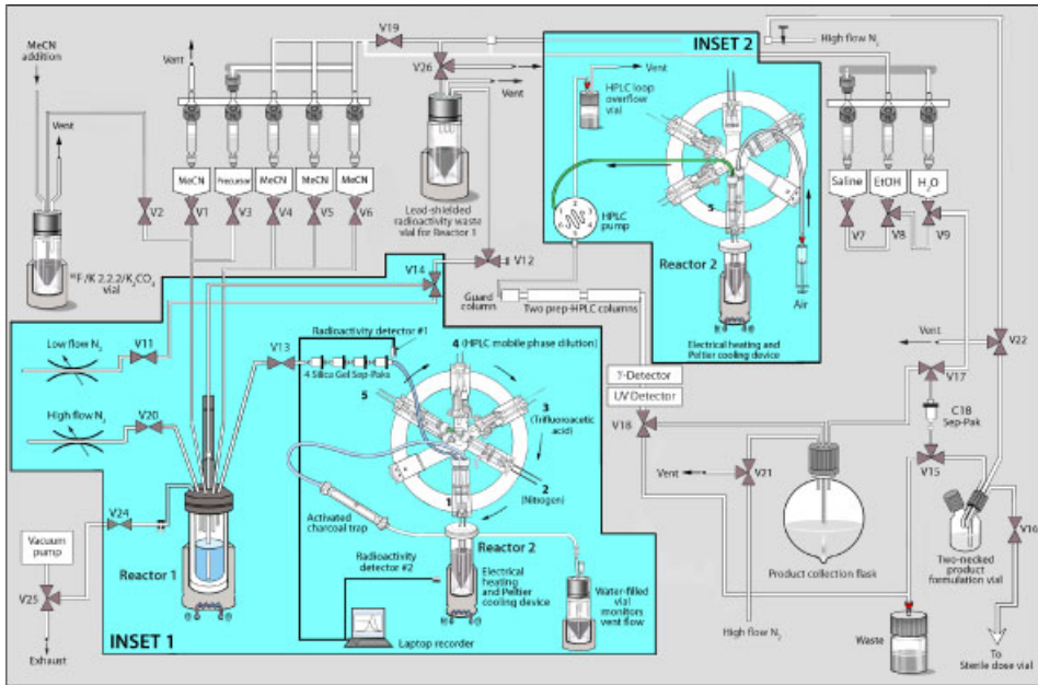
Figure 3. Configuration of TRACERlab FX F-N used to synthesize [ 18 F]fluorobromomethane
